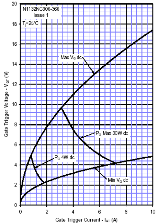
Power curves
