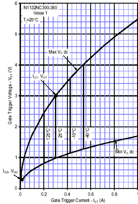
Trigger limits
