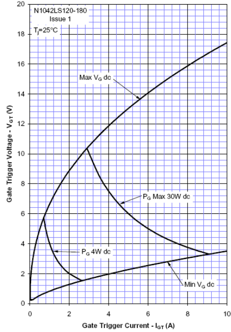
Power curves
