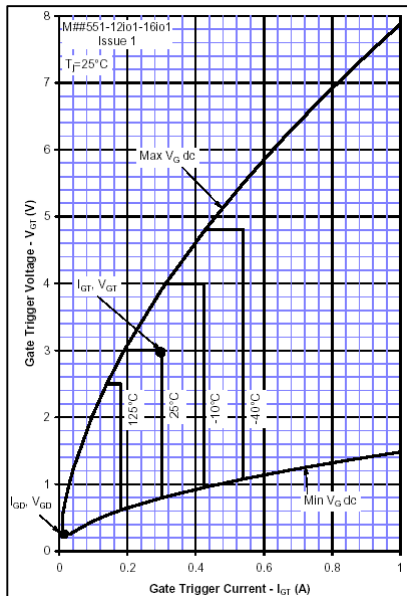
GATE CURRENT
