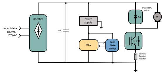
Brushed DC Motor Drive
