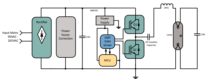
Electronic Lamp Ballast
