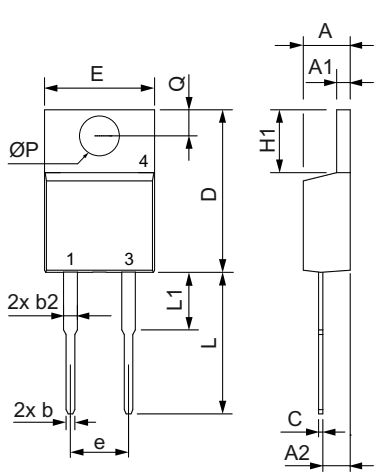
X005b TO-220 AC Weight = 2 g
