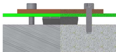
Fig. 4 Mounting example
