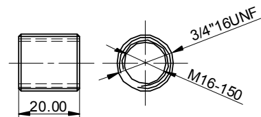
ADPM16-3/4
