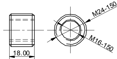
ADPM16-M24
