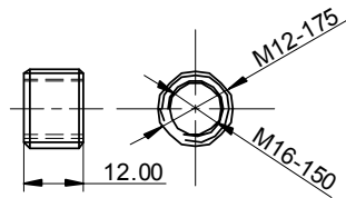
ADPM12-M16
